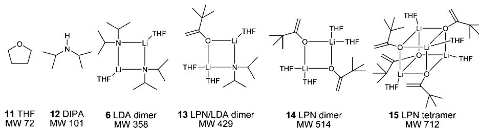
SCHEME 2. LDA and LPN Aggregates in THF
