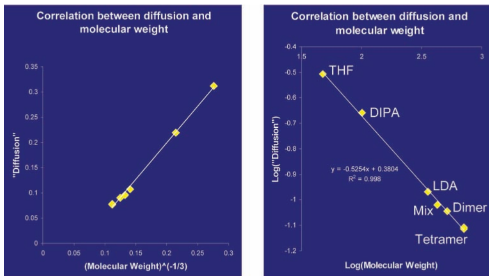
FIGURE 6. ^1\text{H} PFG-DSTE DOSY NMR of LDA/LPN/DIPA in THF- d_6 at -84^\circ\text{C} . Plot of mobility as a function of \text{FW}^a ( a = -1/3 ; left) and log–log plot of mobility as a function of FW (right). (LDA = LDA dimer 6 ; Mix = LPN/LDA mixed dimer 13 ; Dimer = LPN dimer 14 ; Tetramer = LPN tetramer 15 .)
